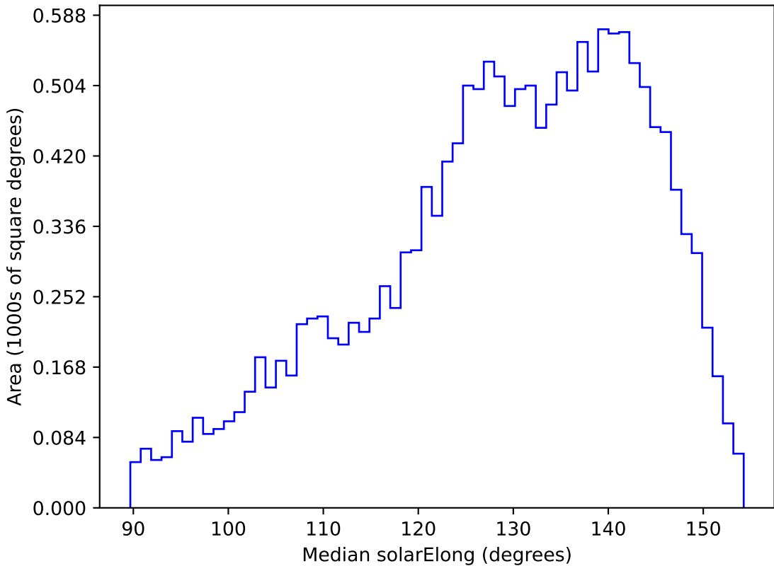
too_elab_r256_d3_griz_v3.4_10yrs WFD g band: Median solarElong
