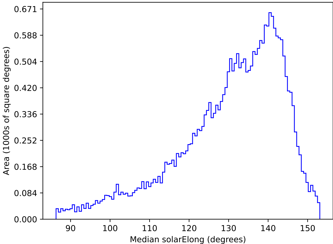
too_elab_r256_d3_griz_v3.4_10yrs All sky r band: Median solarElong
