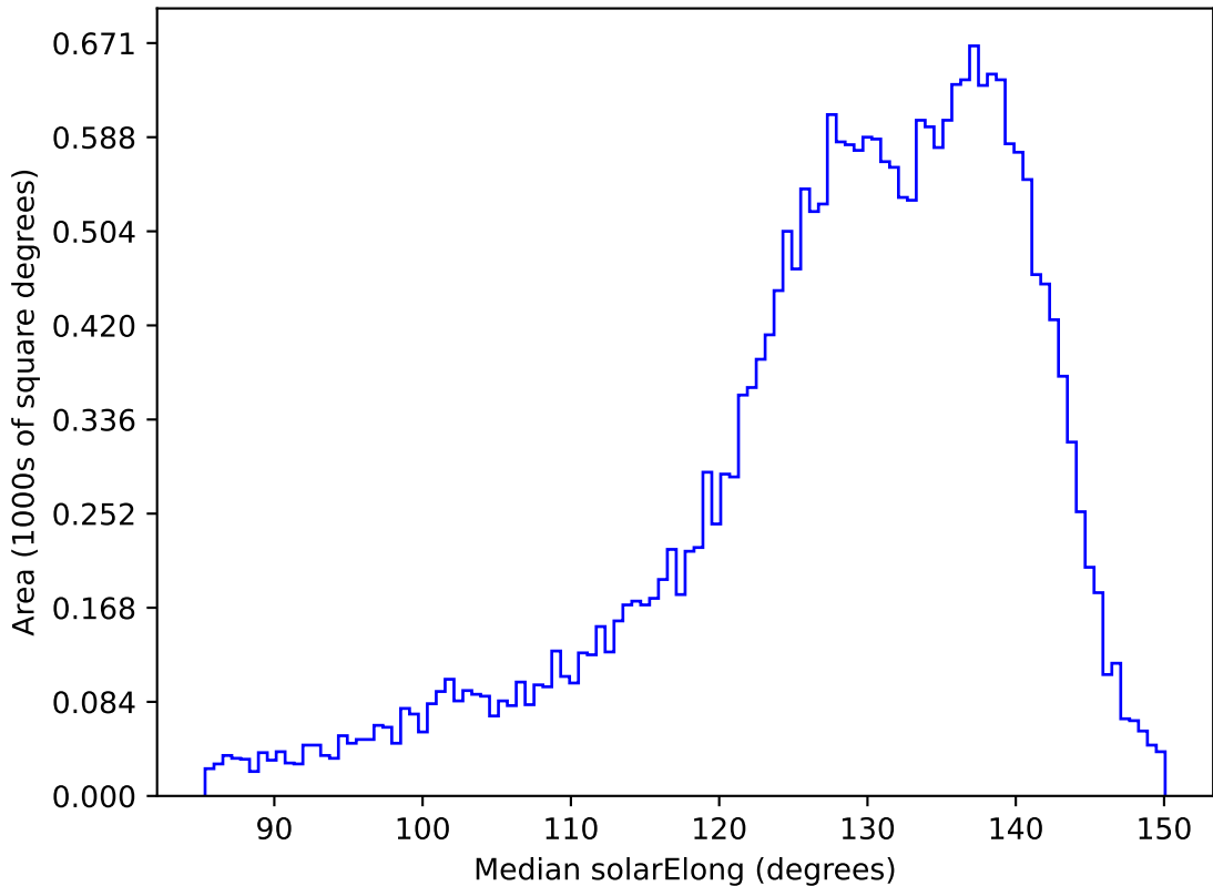
too_elab_r256_d3_griz_v3.4_10yrs All sky i band: Median solarElong
