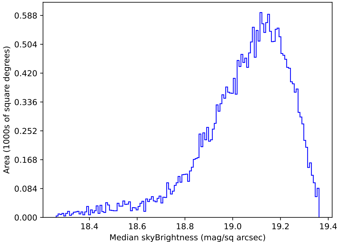
too_elab_r256_d3_griz_v3.4_10yrs Yr 1 z band: Median skyBrightness
