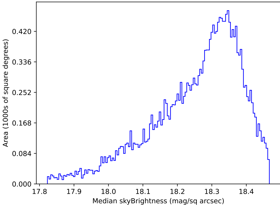
too_elab_r256_d3_griz_v3.4_10yrs Yr 1 y band: Median skyBrightness
