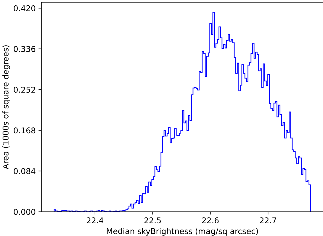
too_elab_r256_d3_griz_v3.4_10yrs Yr 1 u band: Median skyBrightness
