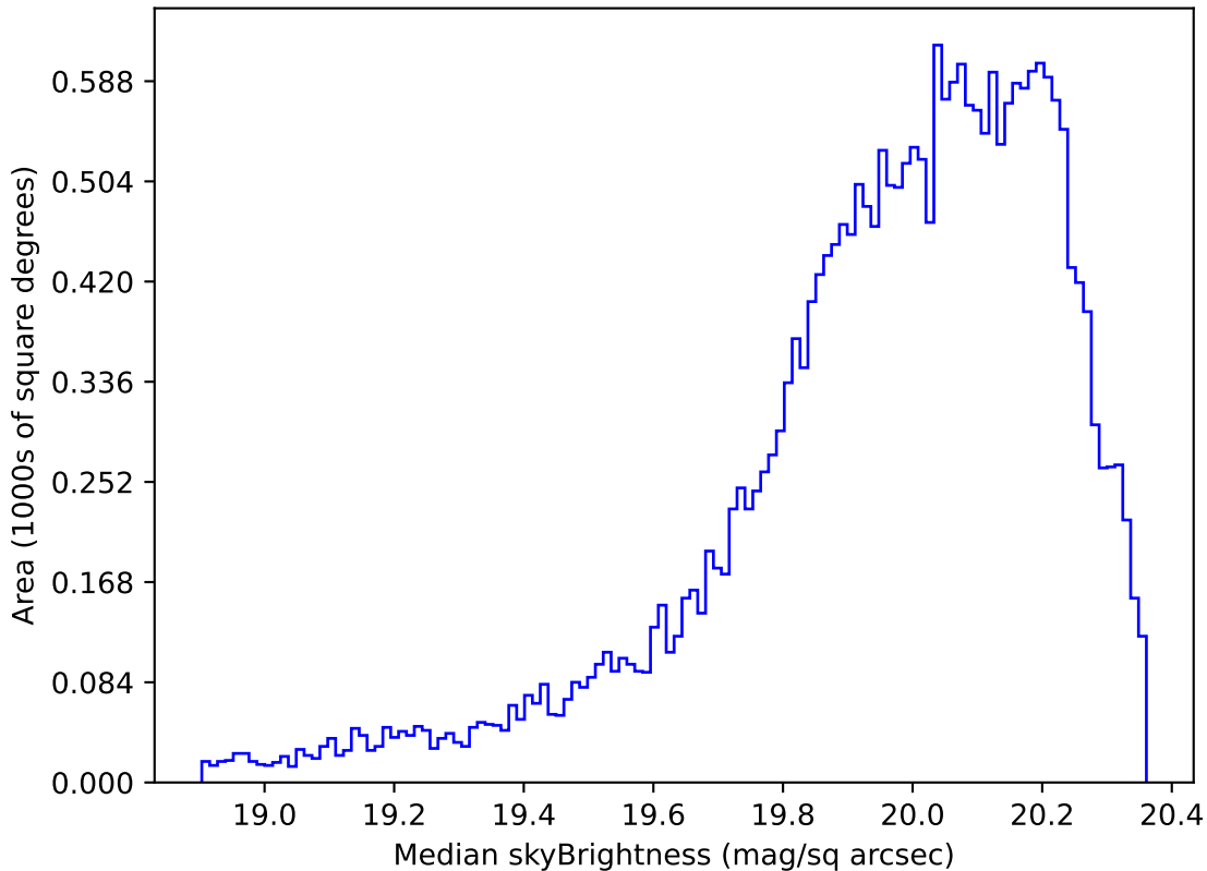
too_elab_r256_d3_griz_v3.4_10yrs Yr 1 i band: Median skyBrightness
