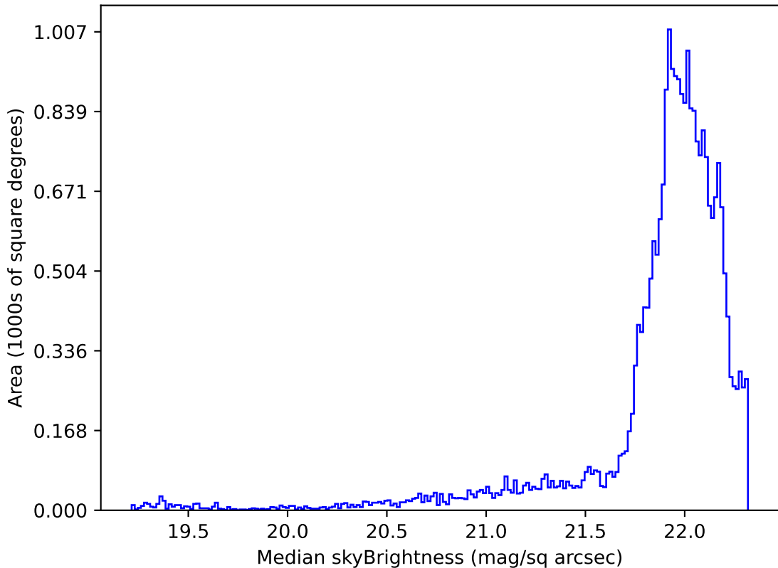
too_elab_r256_d3_griz_v3.4_10yrs Yr 1 g band: Median skyBrightness
