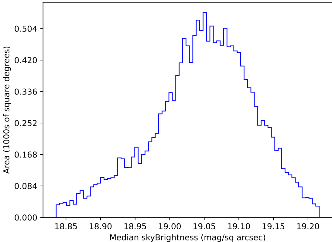
too_elab_r256_d3_griz_v3.4_10yrs WFD z band: Median skyBrightness
