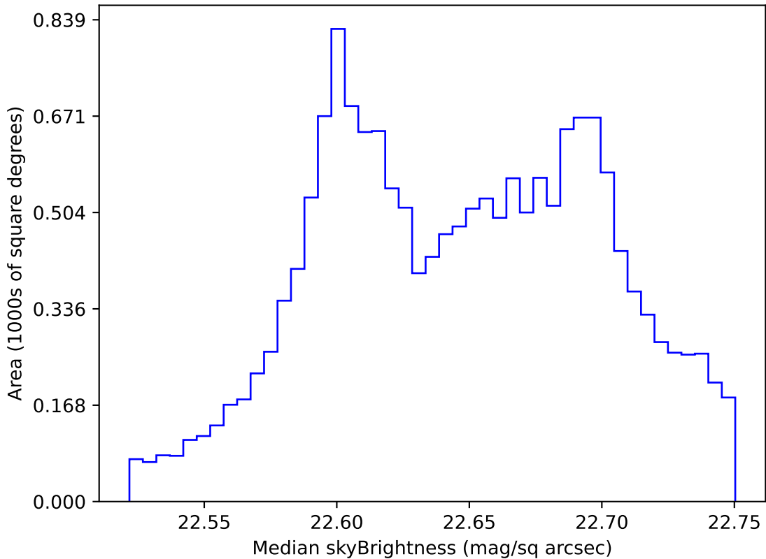
too_elab_r256_d3_griz_v3.4_10yrs WFD u band: Median skyBrightness
