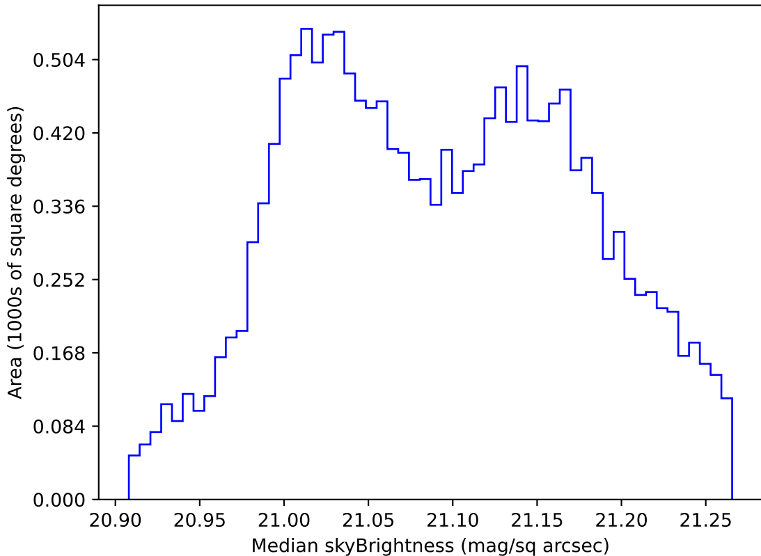
too_elab_r256_d3_griz_v3.4_10yrs WFD r band: Median skyBrightness
