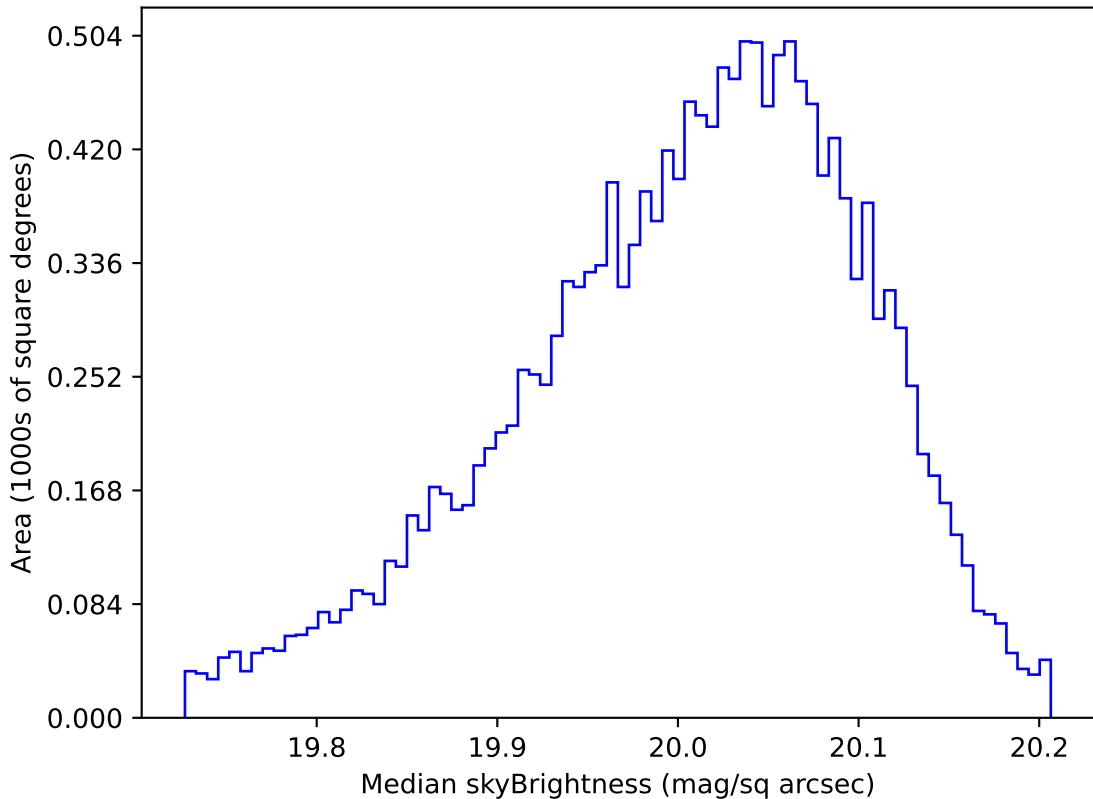
too_elab_r256_d3_griz_v3.4_10yrs WFD i band: Median skyBrightness
