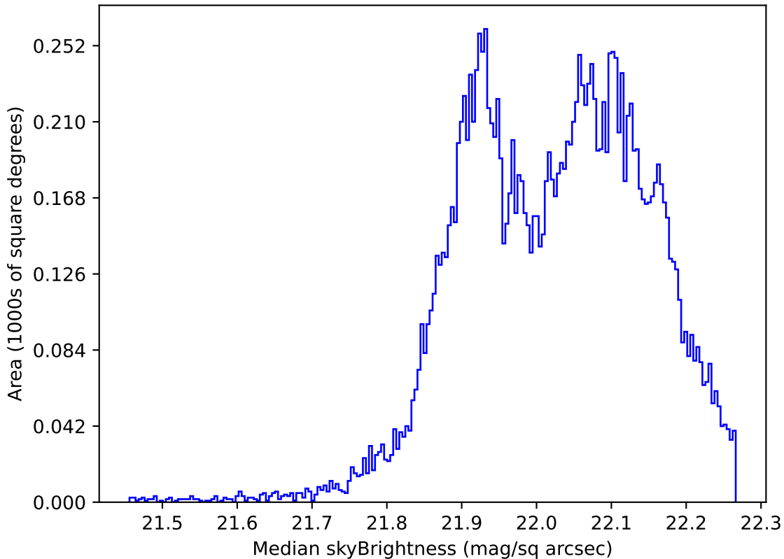
too_elab_r256_d3_griz_v3.4_10yrs WFD g band: Median skyBrightness
