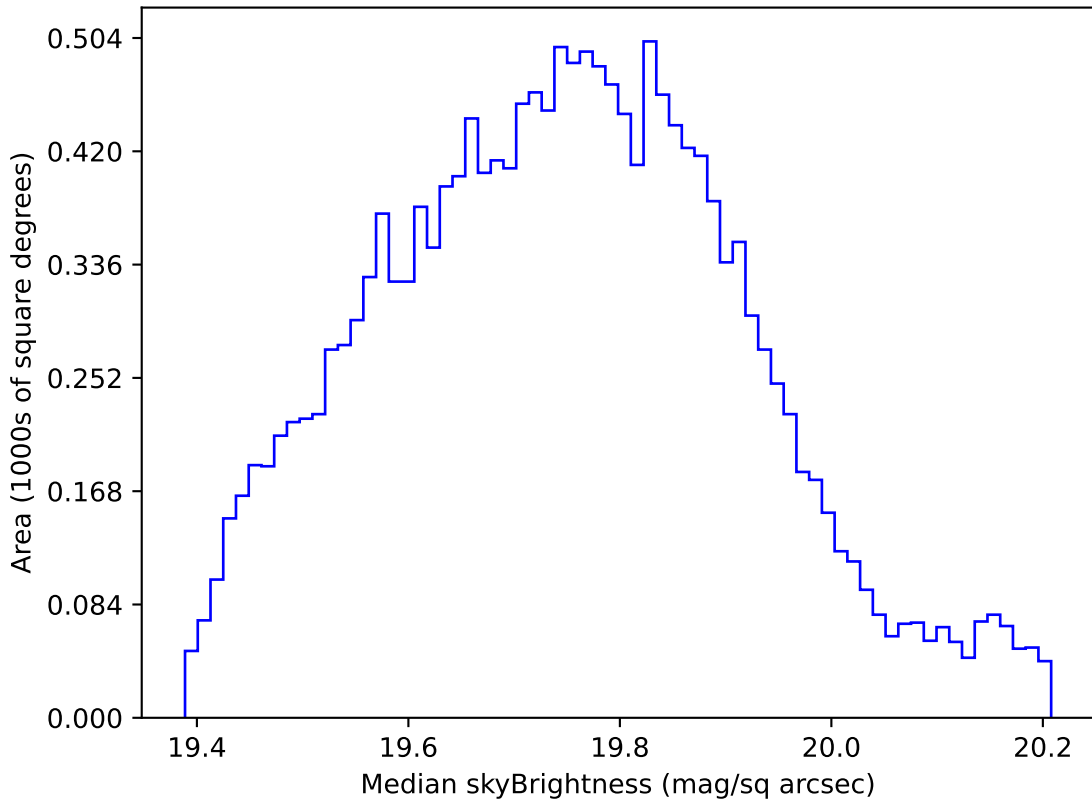
too_elab_r256_d3_griz_v3.4_10yrs WFD all bands: Median skyBrightness
