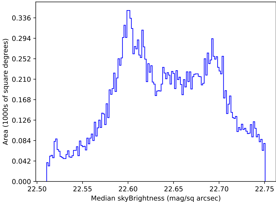
too_elab_r256_d3_griz_v3.4_10yrs All sky u band: Median skyBrightness
