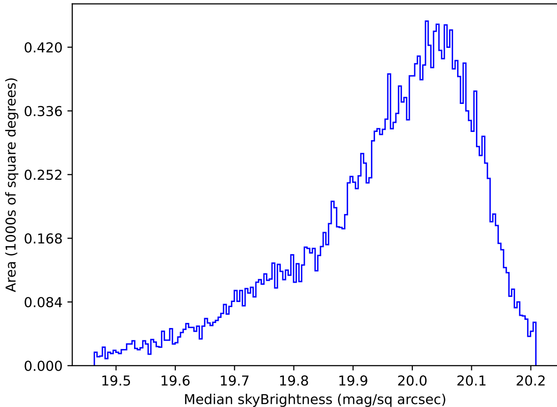
too_elab_r256_d3_griz_v3.4_10yrs All sky i band: Median skyBrightness
