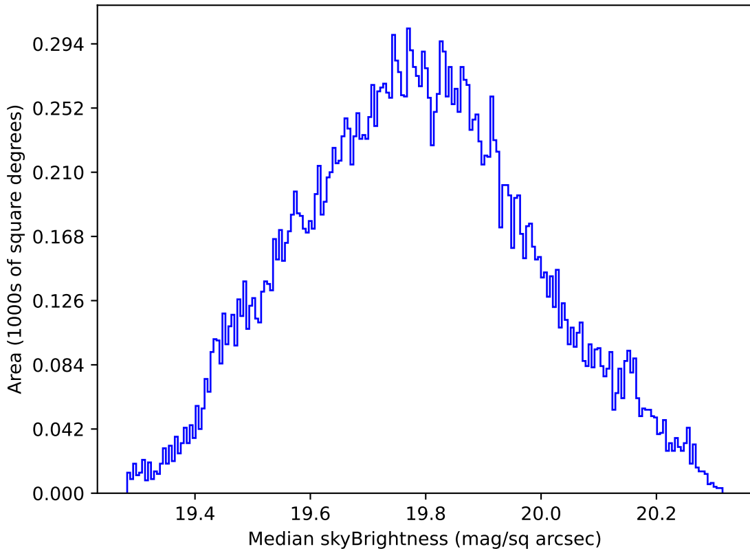
too_elab_r256_d3_griz_v3.4_10yrs All sky all bands: Median skyBrightness
