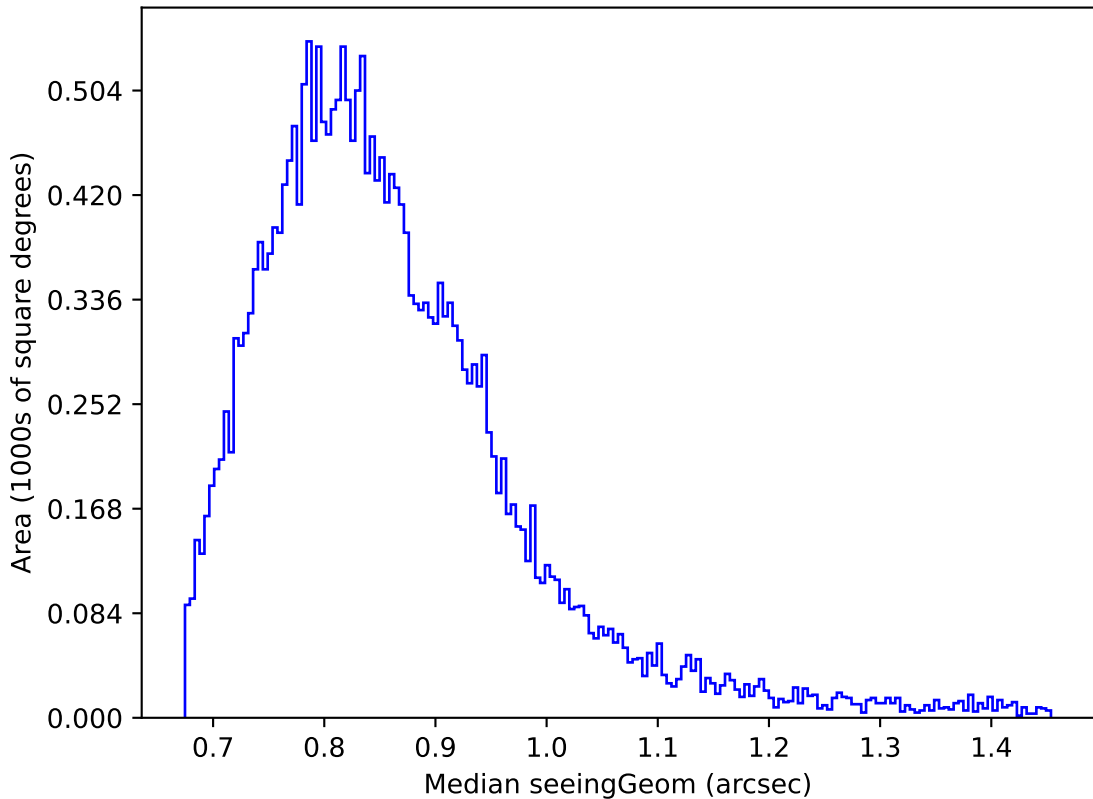
too_elab_r256_d3_griz_v3.4_10yrs Yr 1 z band: Median seeingGeom
