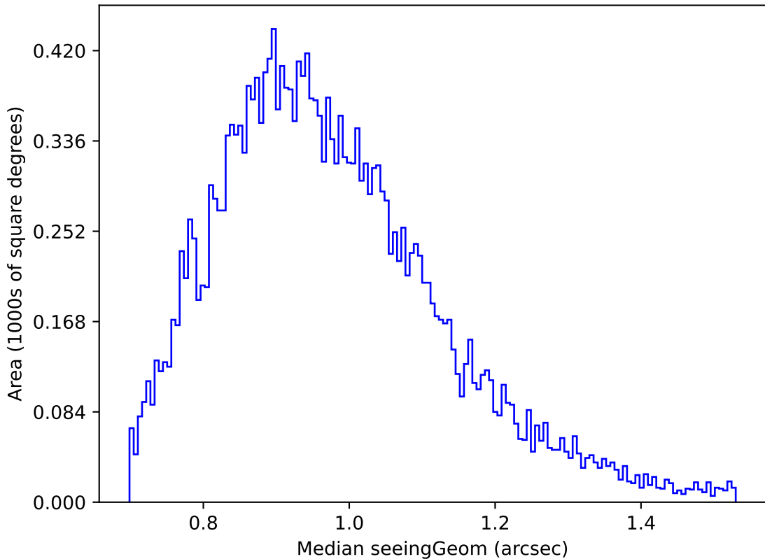
too_elab_r256_d3_griz_v3.4_10yrs Yr 1 u band: Median seeingGeom
