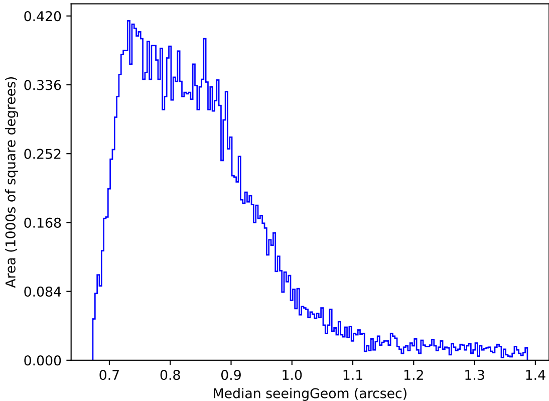
too_elab_r256_d3_griz_v3.4_10yrs Yr 1 i band: Median seeingGeom
