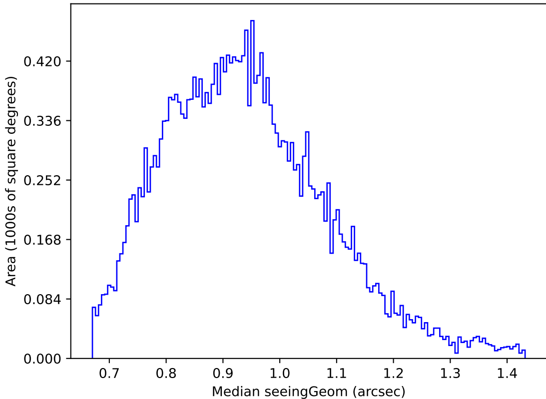
too_elab_r256_d3_griz_v3.4_10yrs Yr 1 g band: Median seeingGeom
