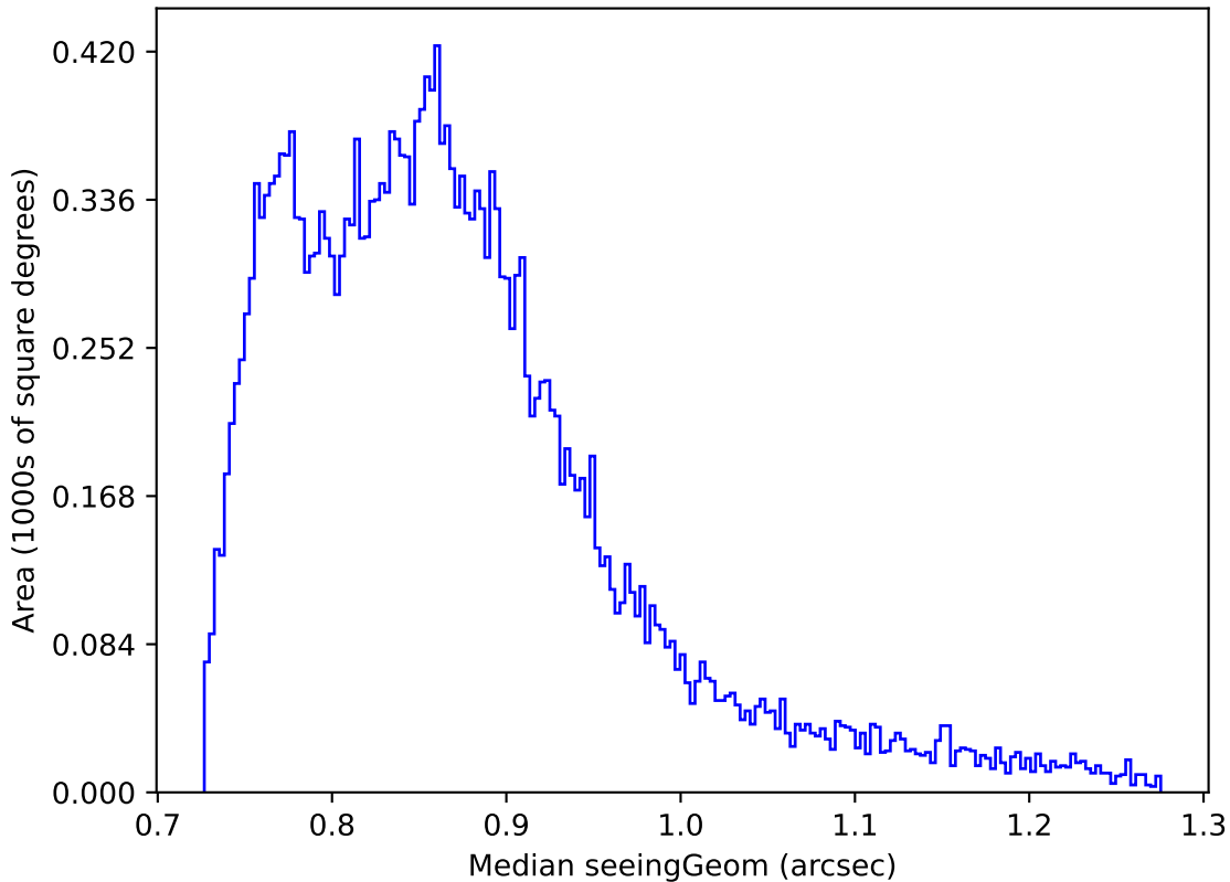
too_elab_r256_d3_griz_v3.4_10yrs Yr 1 all bands: Median seeingGeom
