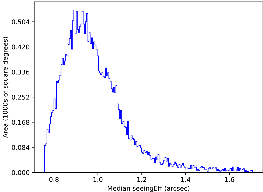
too_elab_r256_d3_griz_v3.4_10yrs Yr 1 z band: Median seeingEff
