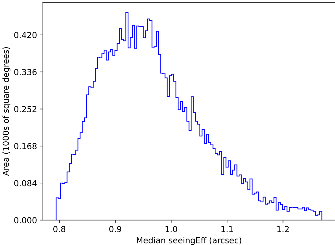
too_elab_r256_d3_griz_v3.4_10yrs Yr 1 y band: Median seeingEff
