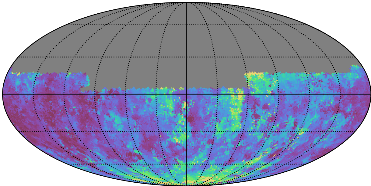
too_elab_r256_d3_griz_v3.4_10yrs Yr 1 u band: Median seeingEff
