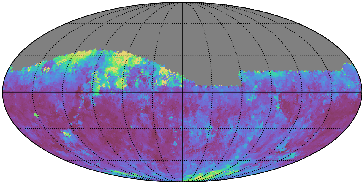
too_elab_r256_d3_griz_v3.4_10yrs Yr 1 i band: Median seeingEff
