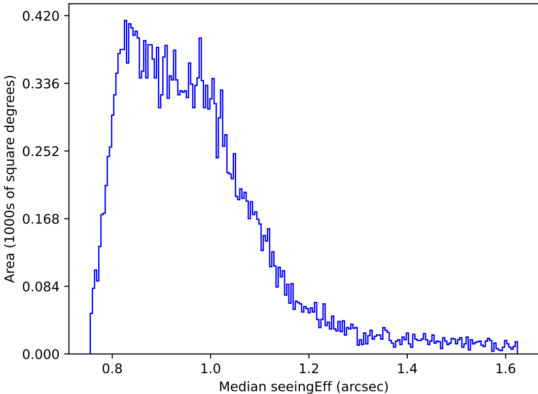
too_elab_r256_d3_griz_v3.4_10yrs Yr 1 i band: Median seeingEff
