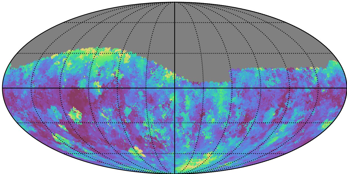
too_elab_r256_d3_griz_v3.4_10yrs Yr 1 g band: Median seeingEff
