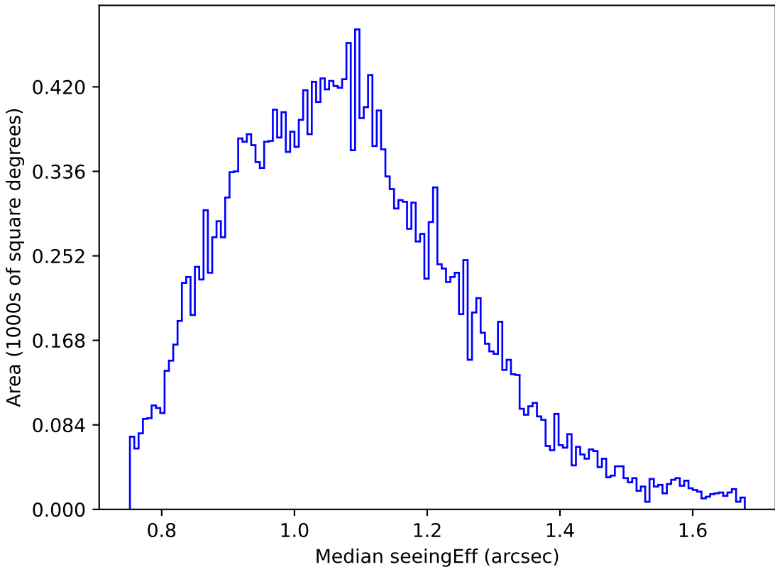
too_elab_r256_d3_griz_v3.4_10yrs Yr 1 g band: Median seeingEff
