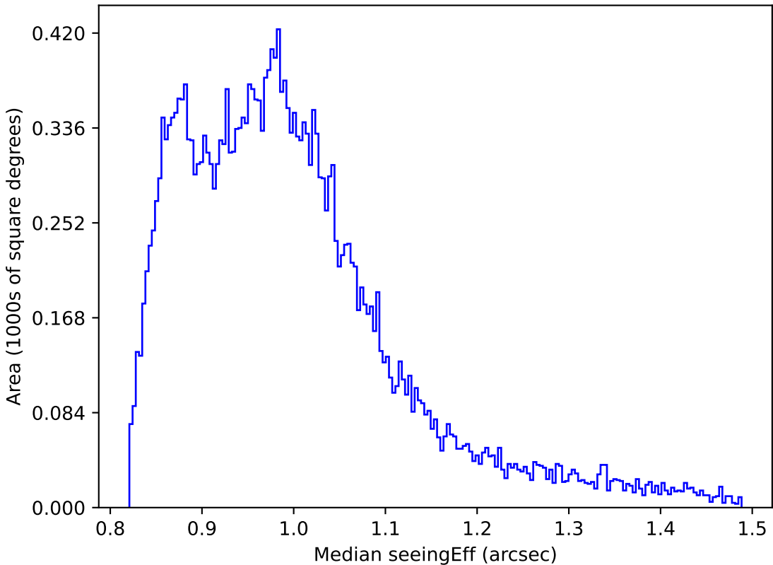
too_elab_r256_d3_griz_v3.4_10yrs Yr 1 all bands: Median seeingEff
