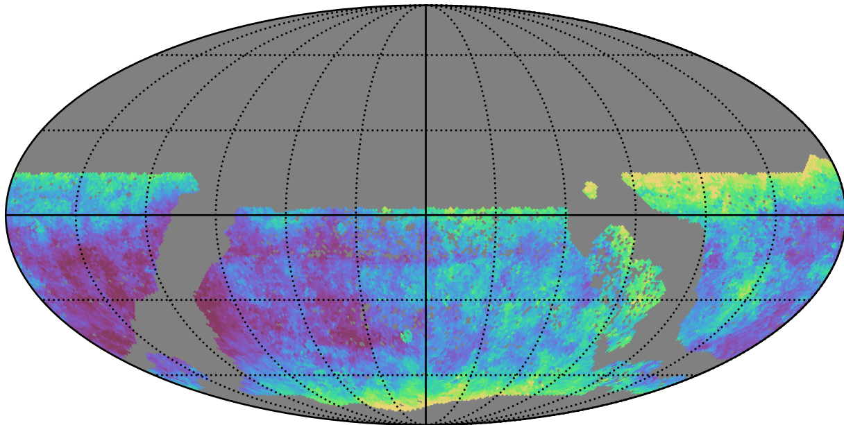
too_elab_r256_d3_griz_v3.4_10yrs WFD y band: Median seeingEff
