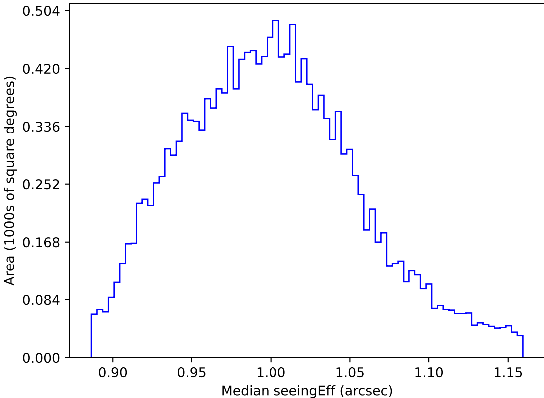
too_elab_r256_d3_griz_v3.4_10yrs WFD y band: Median seeingEff
