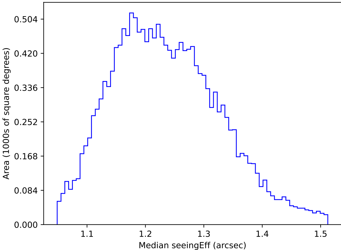
too_elab_r256_d3_griz_v3.4_10yrs WFD u band: Median seeingEff
