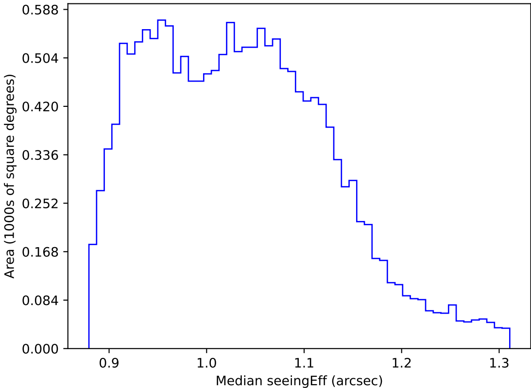
too_elab_r256_d3_griz_v3.4_10yrs WFD r band: Median seeingEff
