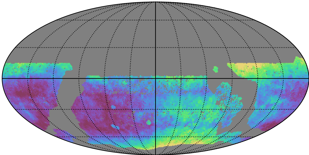
too_elab_r256_d3_griz_v3.4_10yrs WFD i band: Median seeingEff
