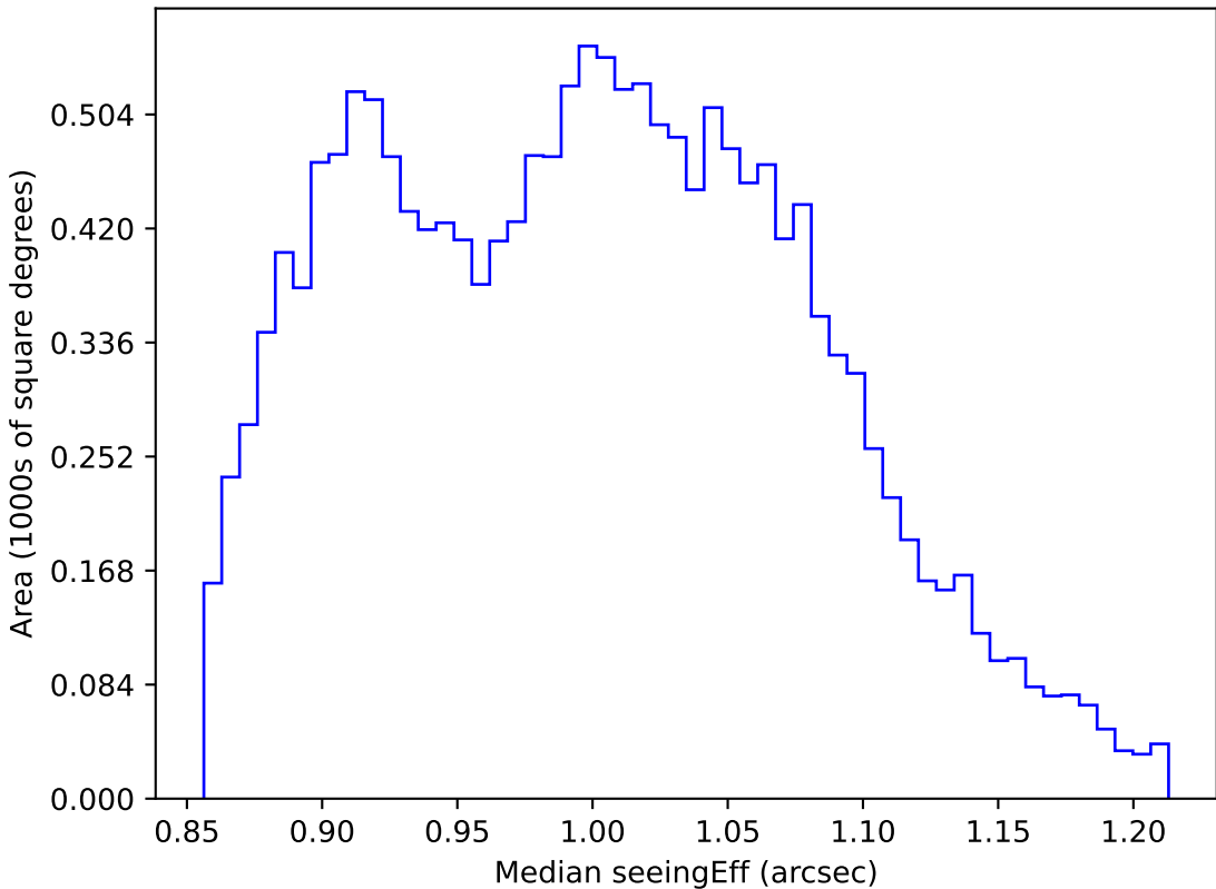
too_elab_r256_d3_griz_v3.4_10yrs WFD i band: Median seeingEff
