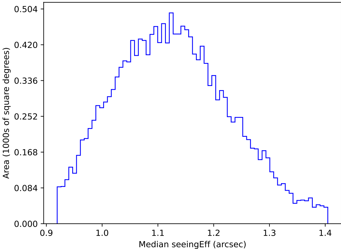
too_elab_r256_d3_griz_v3.4_10yrs WFD g band: Median seeingEff
