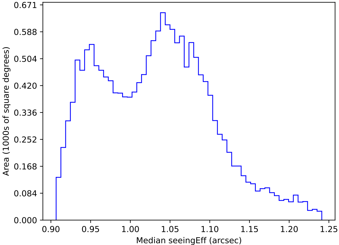
too_elab_r256_d3_griz_v3.4_10yrs WFD all bands: Median seeingEff
