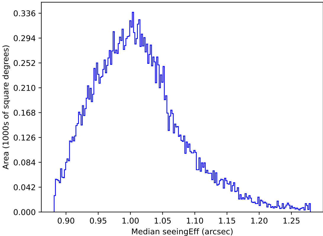
too_elab_r256_d3_griz_v3.4_10yrs All sky y band: Median seeingEff
