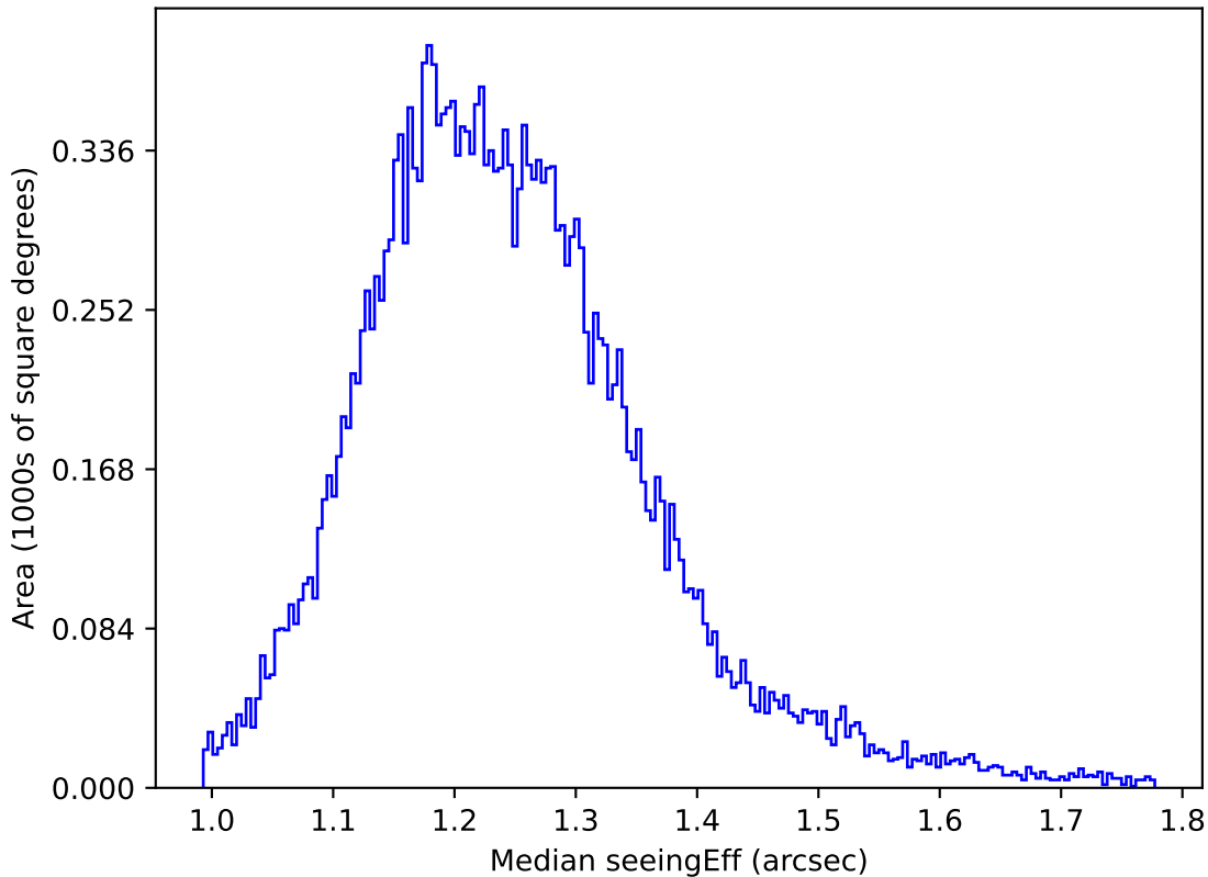
too_elab_r256_d3_griz_v3.4_10yrs All sky u band: Median seeingEff
