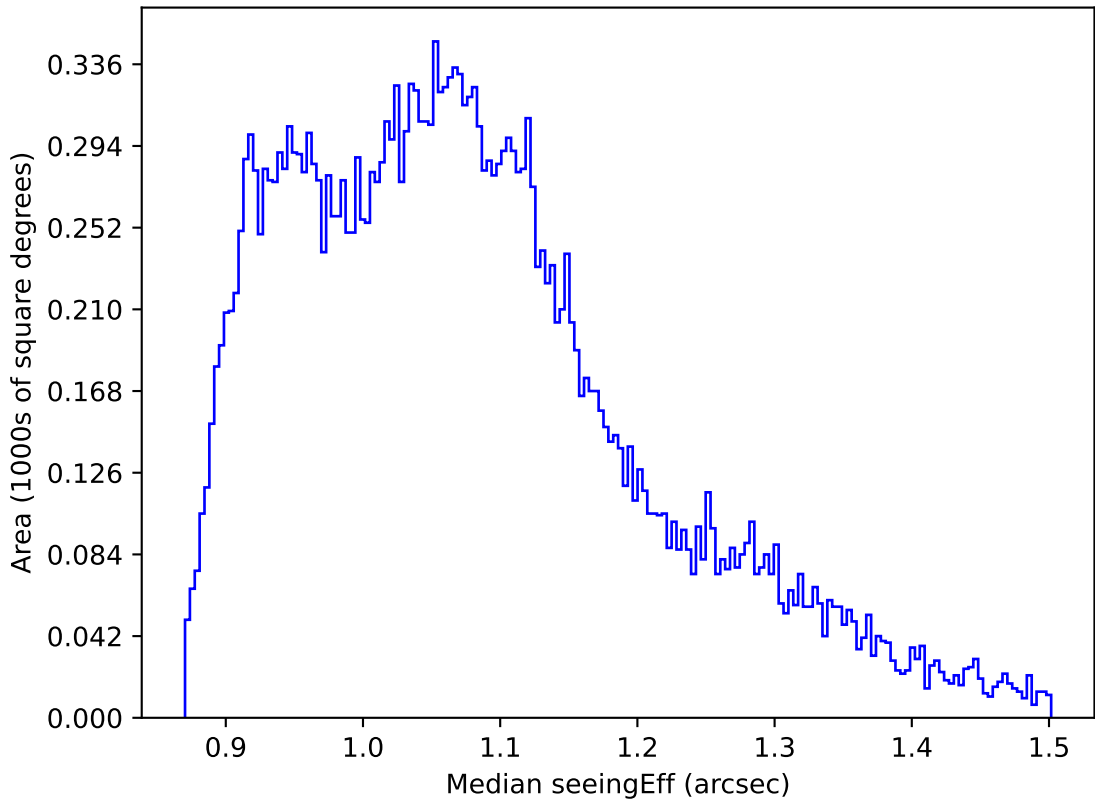
too_elab_r256_d3_griz_v3.4_10yrs All sky r band: Median seeingEff
