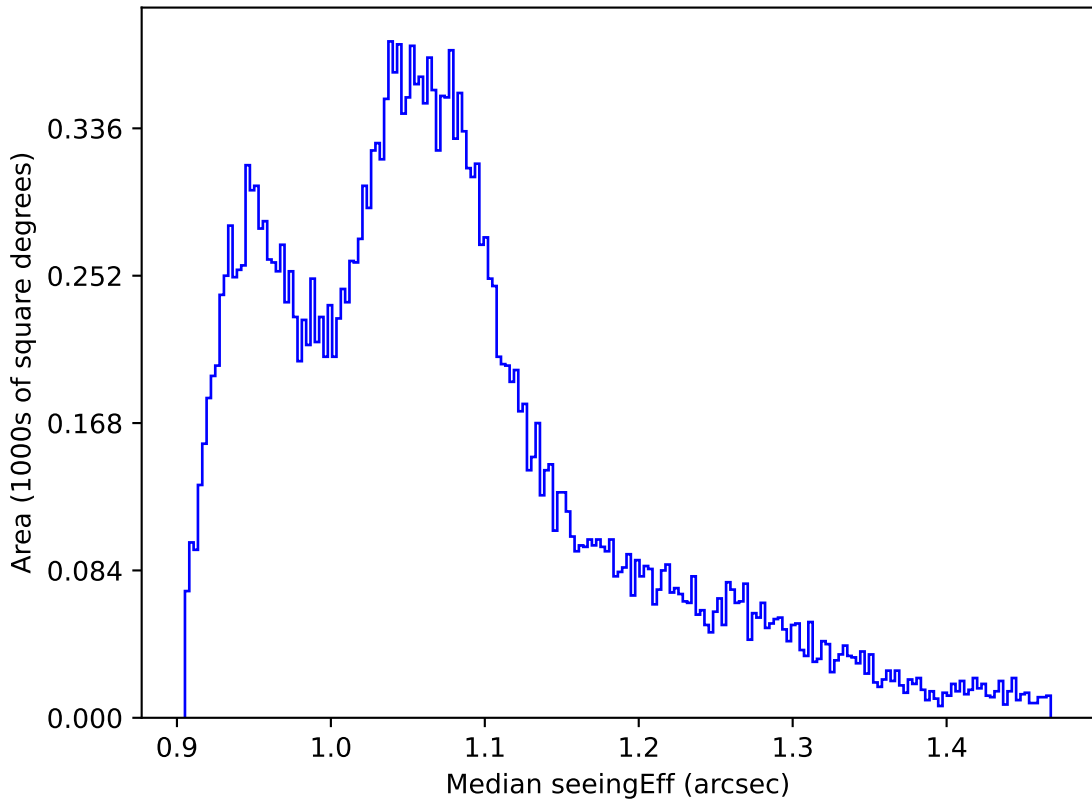
too_elab_r256_d3_griz_v3.4_10yrs All sky all bands: Median seeingEff
