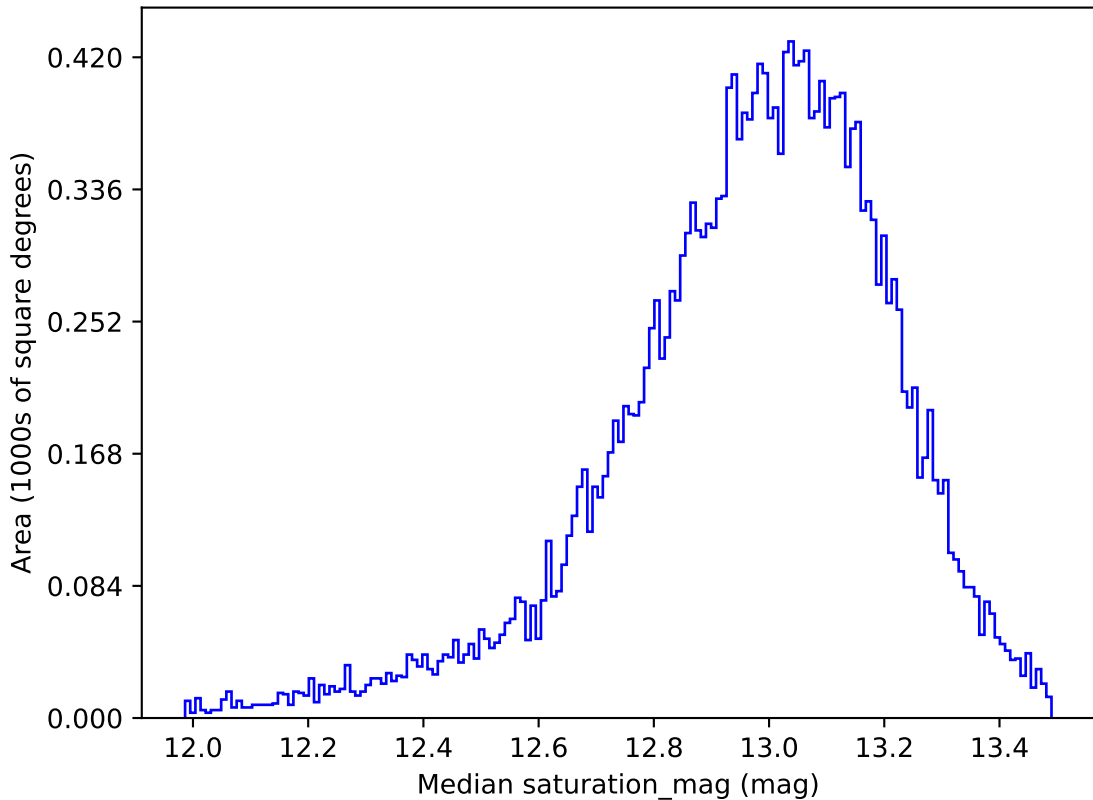
too_elab_r256_d3_griz_v3.4_10yrs All sky u band: Median saturation_mag
