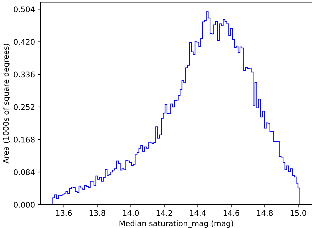
too_elab_r256_d3_griz_v3.4_10yrs All sky g band: Median saturation_mag
