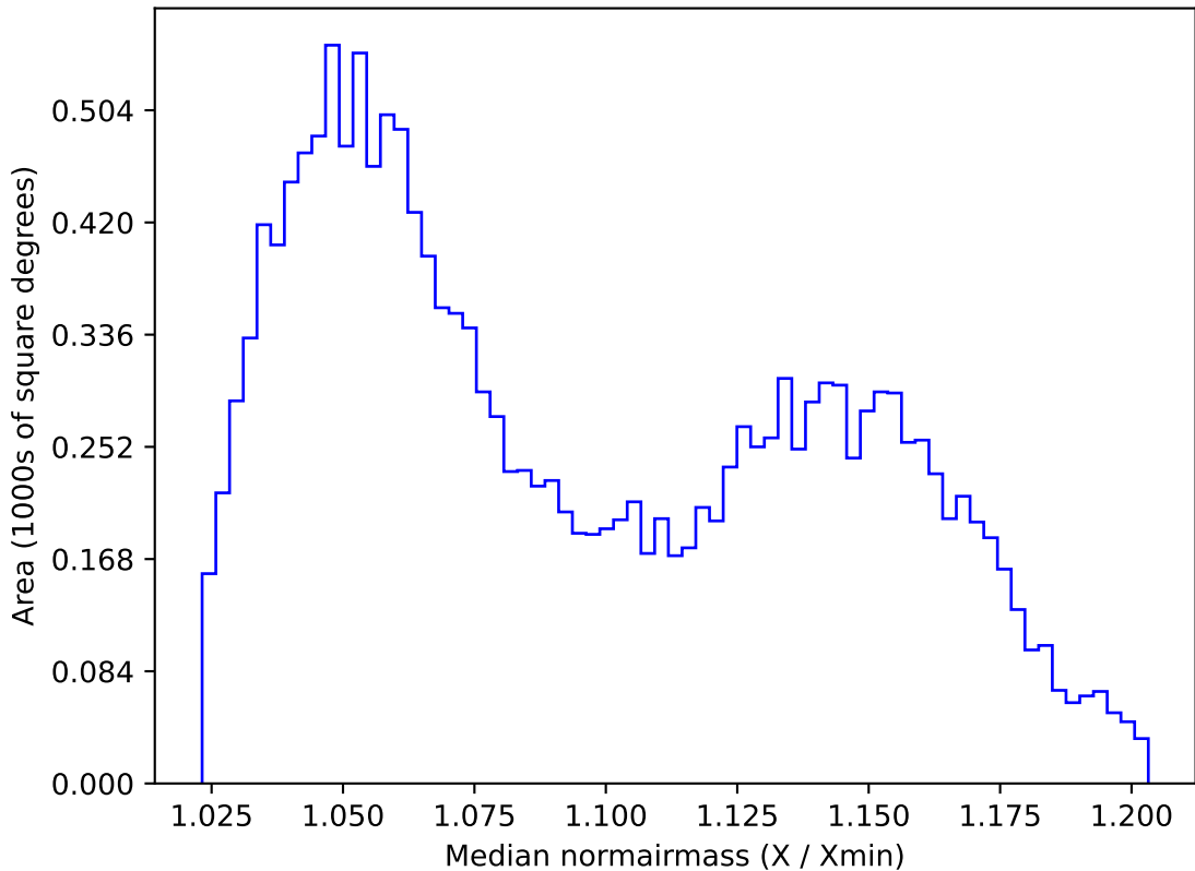
too_elab_r256_d3_griz_v3.4_10yrs WFD z band: Median normairmass
