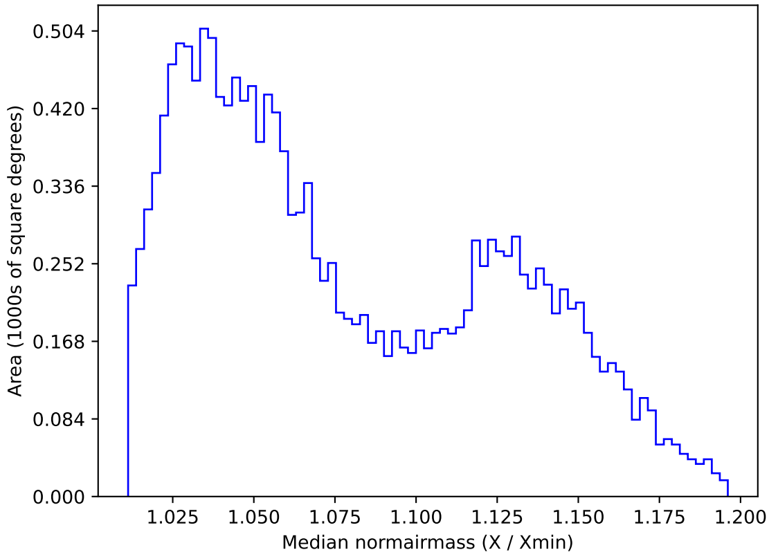
too_elab_r256_d3_griz_v3.4_10yrs WFD u band: Median normairmass
