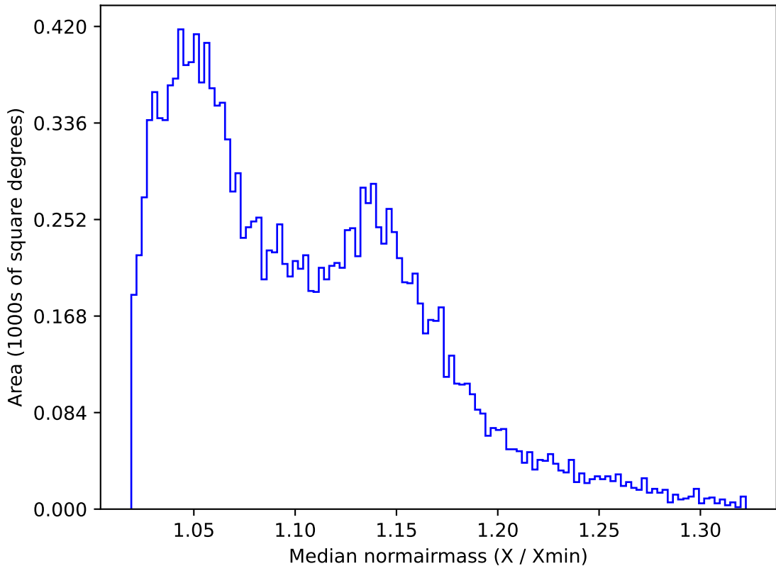
too_elab_r256_d3_griz_v3.4_10yrs WFD g band: Median normairmass
