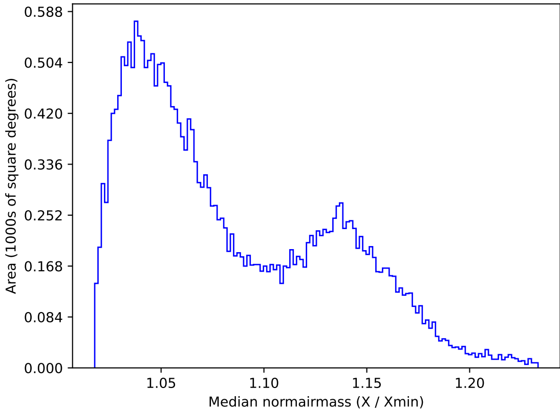
too_elab_r256_d3_griz_v3.4_10yrs All sky i band: Median normairmass
