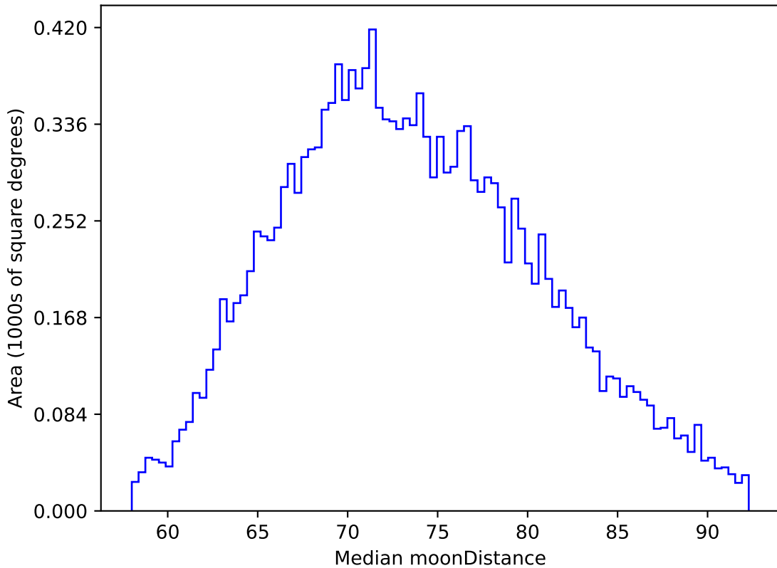
too_elab_r256_d3_griz_v3.4_10yrs WFD z band: Median moonDistance
