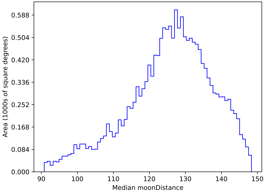
too_elab_r256_d3_griz_v3.4_10yrs WFD u band: Median moonDistance
